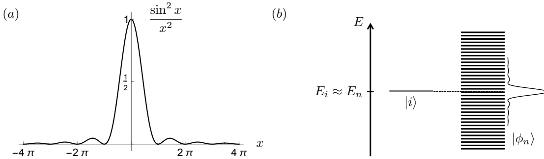
Figure 3: Time-dependent perturbation theory. (a) Function \sin^2 x/x^2 involved in the transition probability. (b) A single state |i\rangle coupled to a quasi-continuum of states |\phi_n\rangle . Only the states |\phi_n\rangle with an energy close to E_i contribute significantly to the transition.
